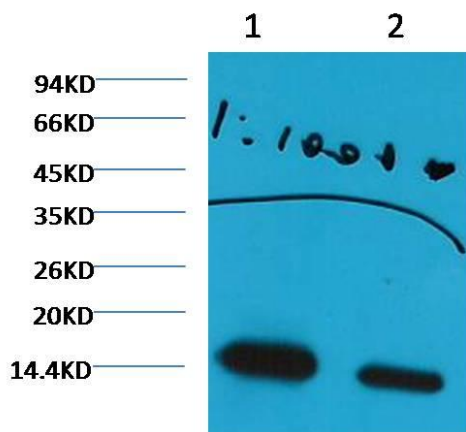
Western blot analysis of HeLa with Histone H3 (di methyl K27) (1E10) Mouse MAb diluted at 1) 1:1,000 2) 1:3,000
