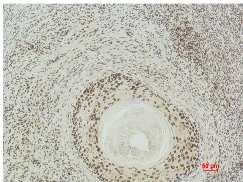
Immunohistochemical analysis of paraffin-embedded Human Skin using Histone H3(di methyl K27) Mouse mAb diluted at 1:500.
